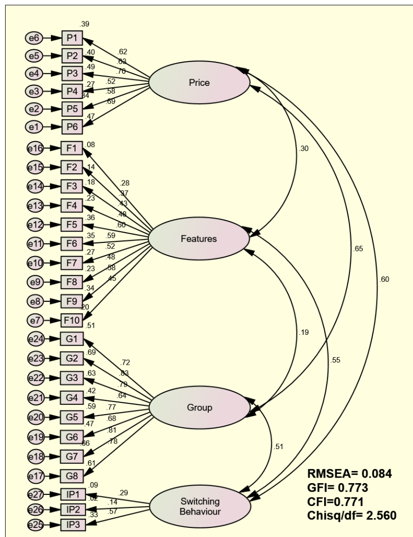
Fig 1: Measurement Model
