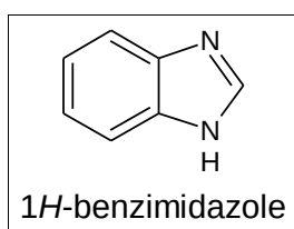
Fig 1: Benzimidazole heterocyclic nucleus
